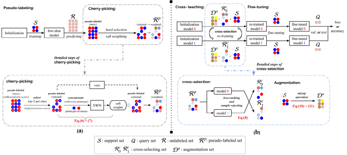
Fig. 2. Details of applying LTTL to a single (2-class, 2-shot) task in the inner-loop. (a) Pseudo-labeling and cherry-picking operations for processing the unlabeled set R . Hard-selection and soft weighting are subsequently used in cherry-picking to select informative samples. (b) Cross-teaching operation for rejecting more noisy labels. Double-branch classifiers with indexes 0 and 1 are used in this process, which reject noisy labeled samples according to the loss values for each other. After re-training with the pseudo-labeled set R^p , the classifiers are further fine-tuned with the clean set S to avoid the drifting problem.
