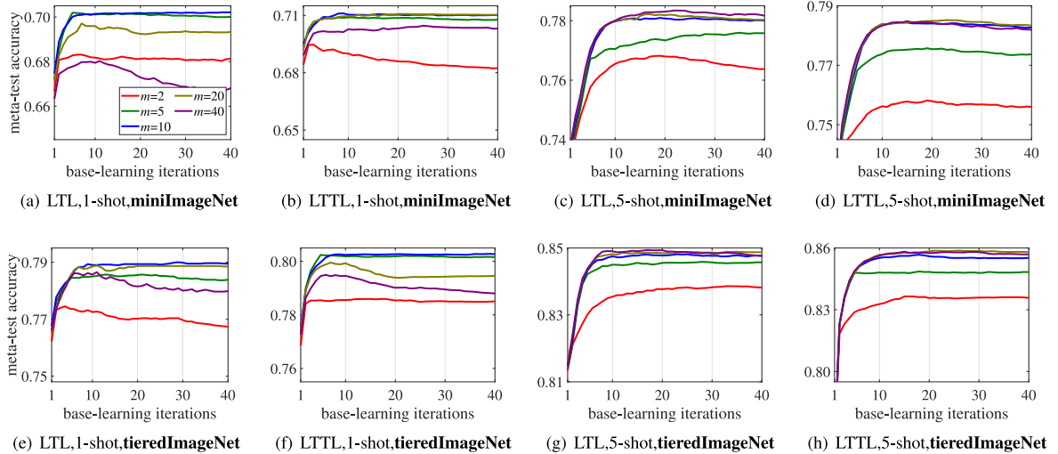
Fig. 3. Classification accuracy using different numbers of re-training steps, e.g. m = 2 means using 2 steps for re-training and 38 steps (40 steps in total) for fine-tuning at every recursive stage. Each curve shows the results obtained at the final recursive stage. LTL: our method (LST) in the conference version (Li et al., 2019); LTT: the new proposed teaching and learning framework.
