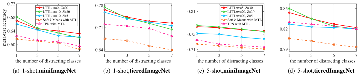
Fig. 4. Classification accuracy with different numbers of distracting classes on the miniImageNet and tieredImageNet. We evaluate our proposed LTTL by using different values for re-training steps m and hard-selection number Z . Noting that (a) and (b) share legend, and (c) and (d) share legend.
