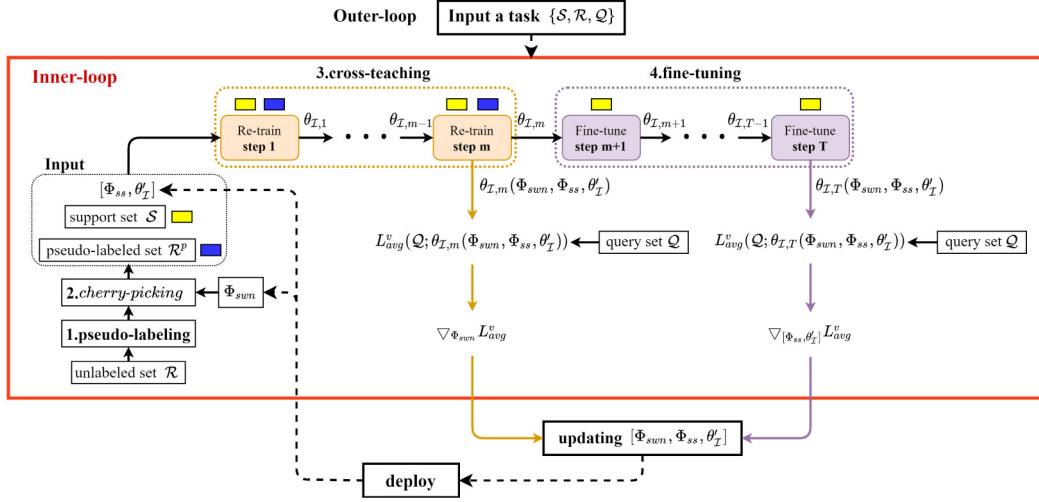
Fig. 1. The two-loop training procedure of LTTL. cherry-picking is used to process unlabeled samples for the inner-loop process. The updating procedure of inner-loop contains m steps of re-training and T - m steps of fine-tuning. For re-training process, cross-teaching is used to deal with pseudo-labeled data obtained from cherry-picking . The meta-parameters [\Phi_{sum}, \Phi_{ss}, \theta_X] are updated in the outer-loop by using the validation losses L^v_{avg} . (For interpretation of the references to color in this figure legend, the reader is referred to the web version of this article.)
