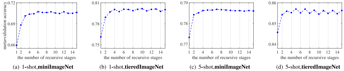
Fig. 5. Meta-validation accuracy achieved at different numbers (1–15) of recursive stages, on the miniImageNet and tieredImageNet datasets.
